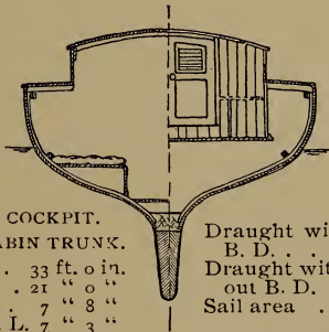
SEAWANHAKA KNOCKABOUT.
